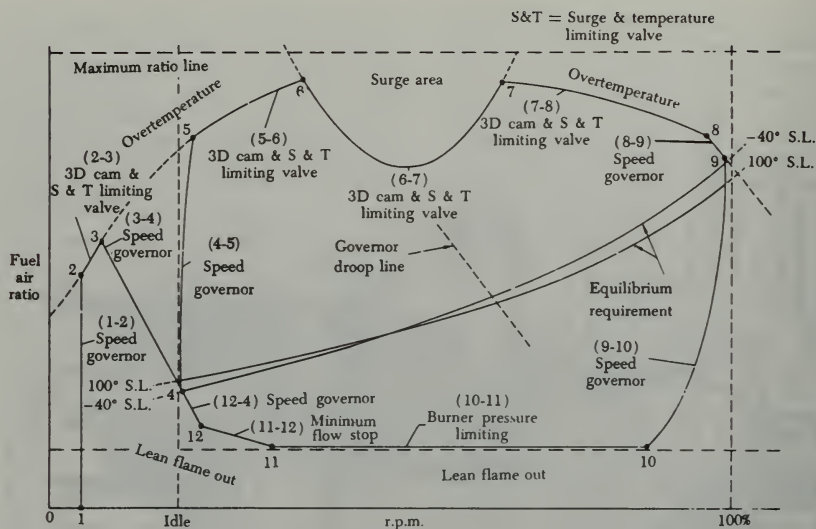
FIGURE 3-47. Engine operating conditions (equilibrium curve).
